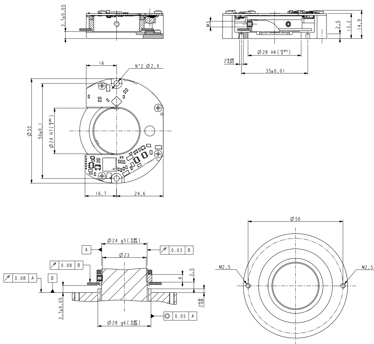
AMM5A - Mounting requirements
