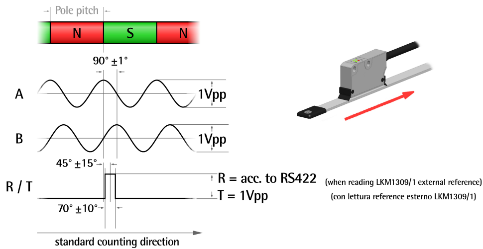
Figure 7 - Output signals
